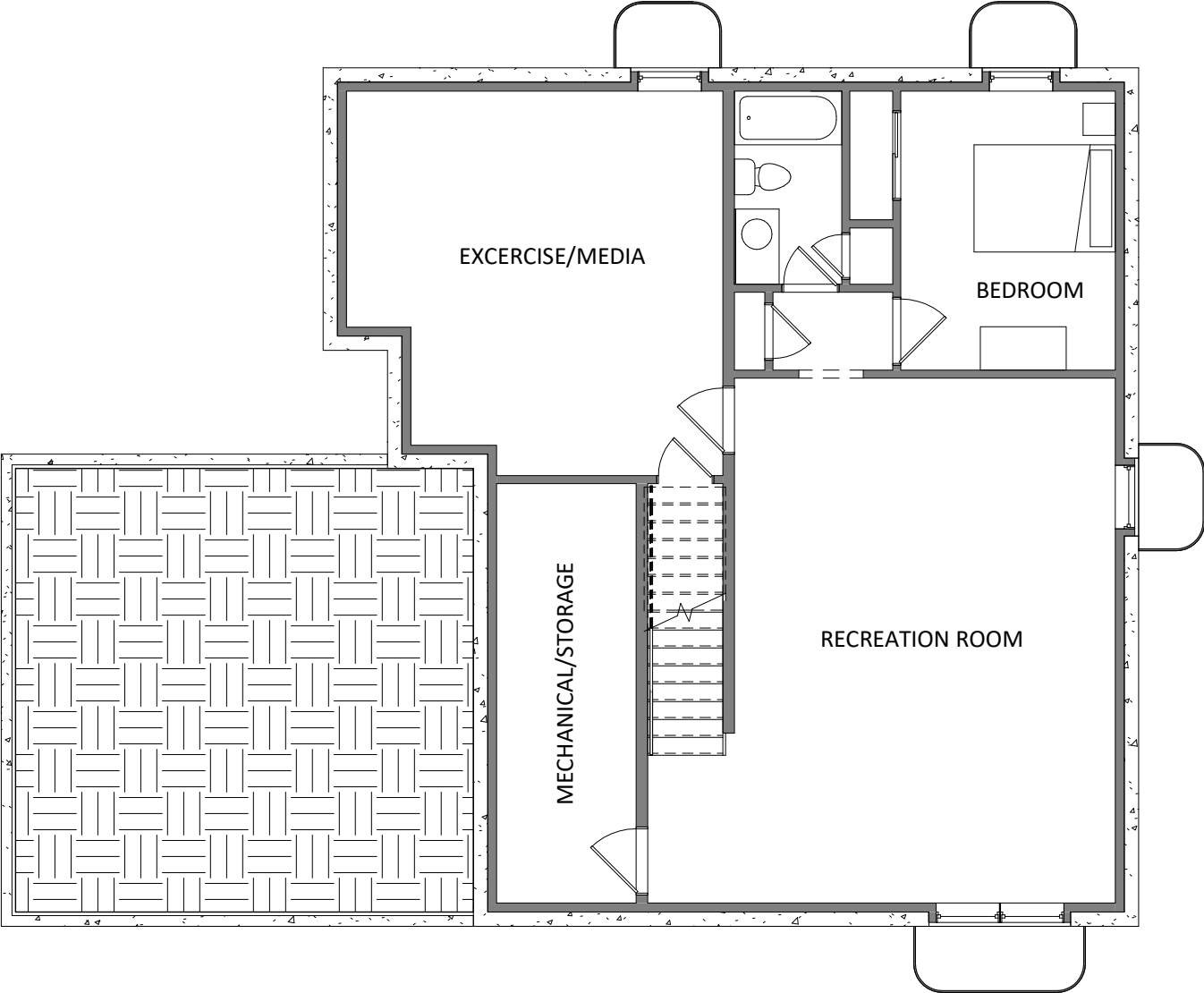
BASEMENT LEVEL FLOOR PLAN
